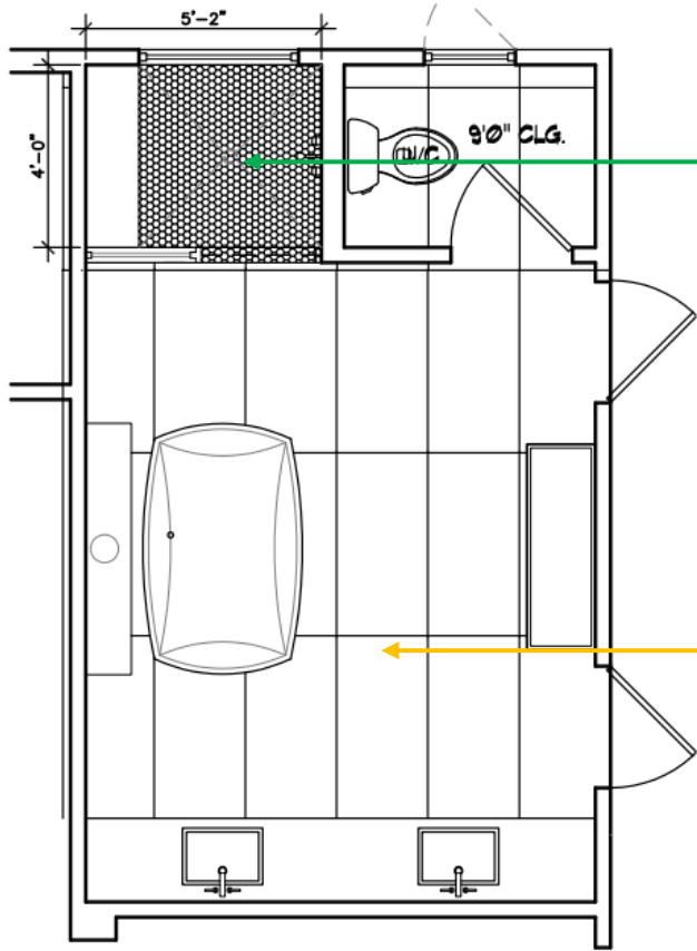
MASTER BATHROOM FLOOR PLAN
